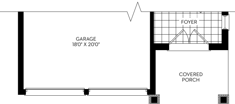
MAIN FLOOR B
