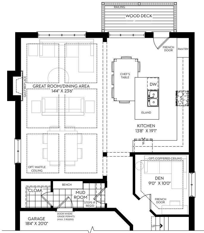
MAIN FLOOR 2 OPTIONAL LAYOUT
