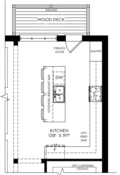
MAIN FLOOR 2 ALTERNATE KITCHEN
