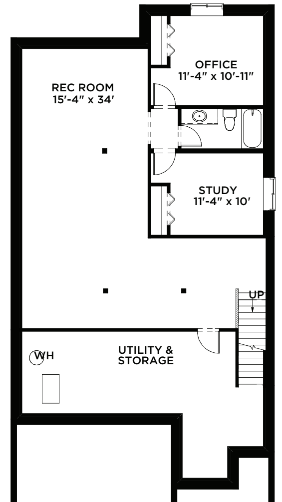
Basement development for the standard double garage. Adds 1,086 sq.ft.
