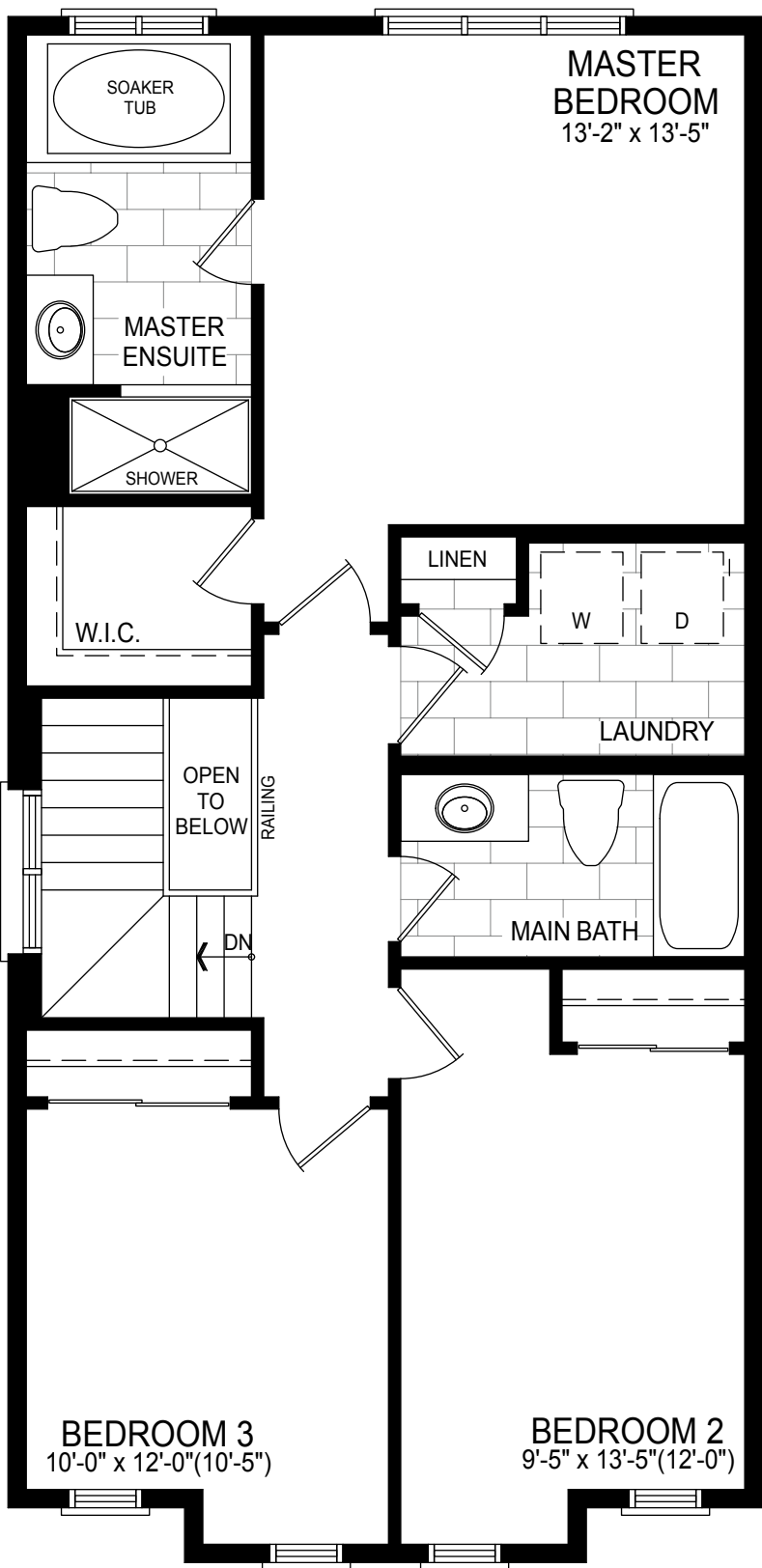
SECOND FLOOR PLAN STYLE A
