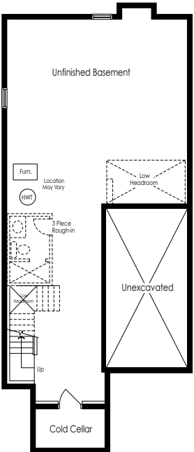
Basement Elevation A
