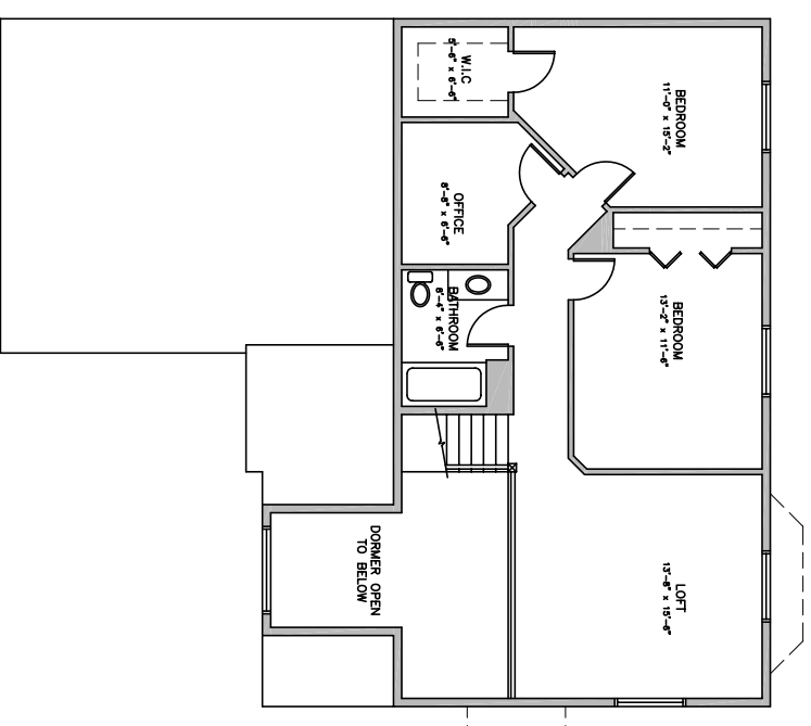
SECOND STOREY PLAN
