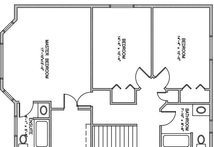
SECOND STOREY PLAN
