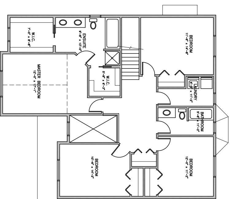
SECOND STOREY PLAN
