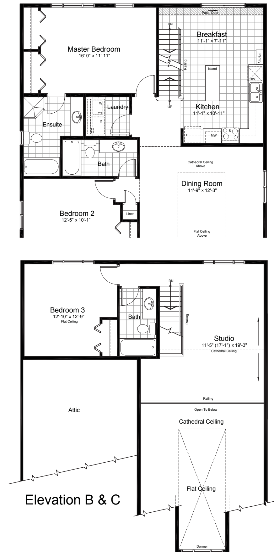
GROUND FLOOR WITH LOFT
