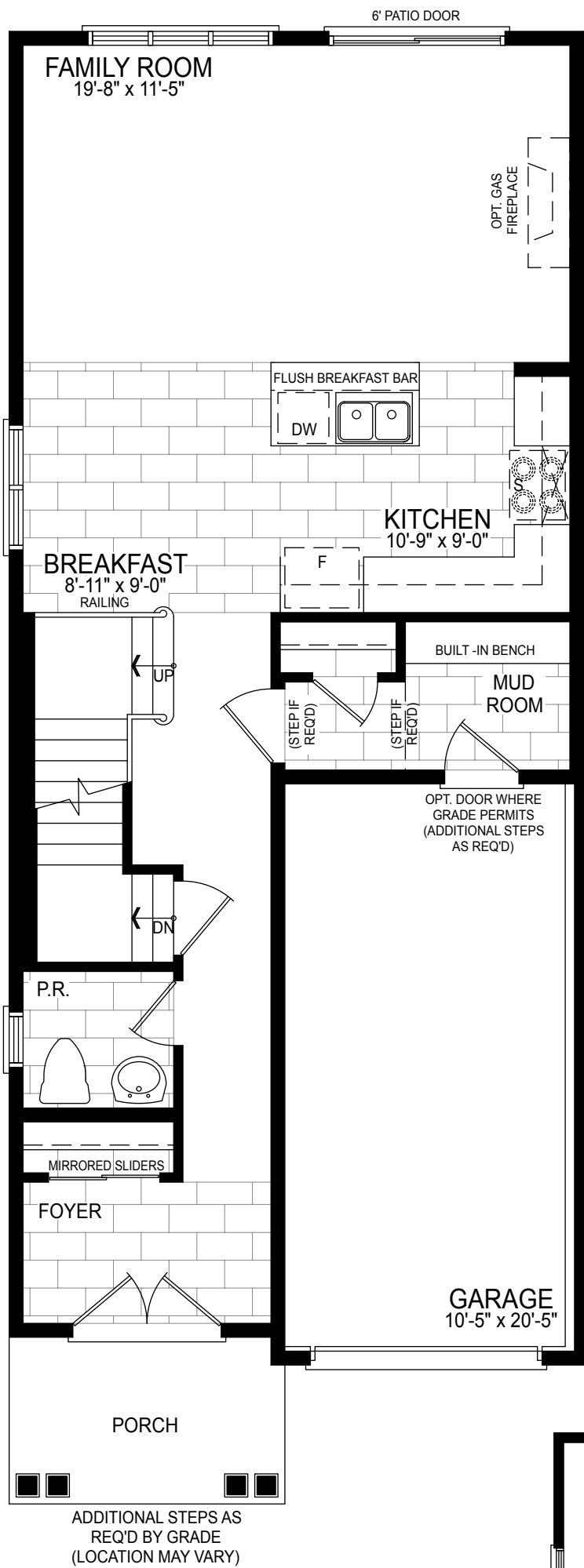
GROUND FLOOR PLAN STYLE A
