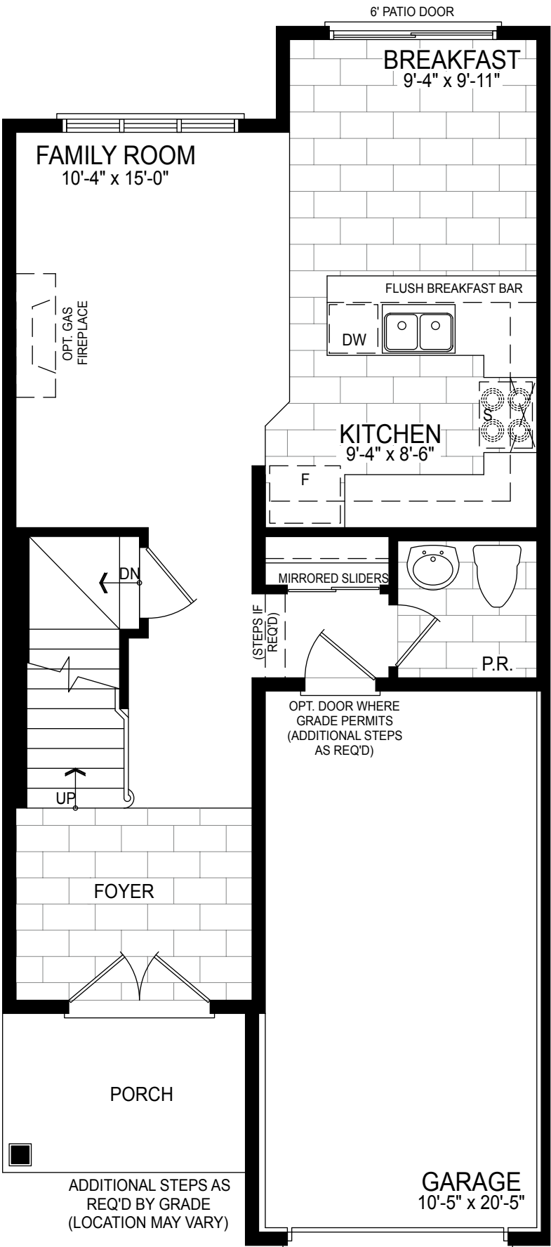
GROUND FLOOR PLAN STYLE A
