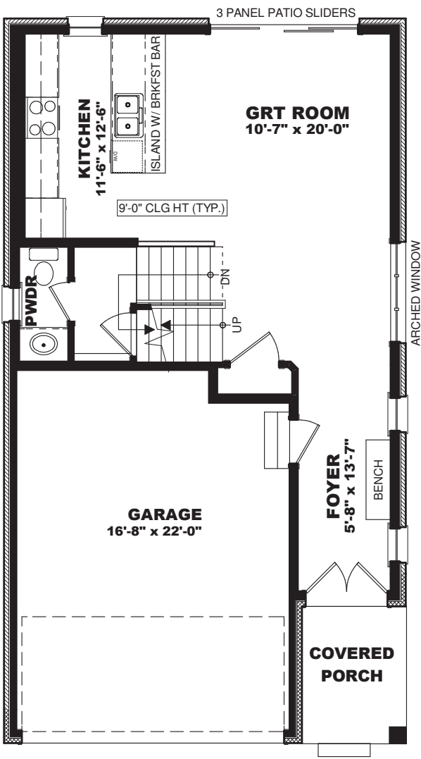
MAIN FLOOR PLAN - 637 SQ. FT
