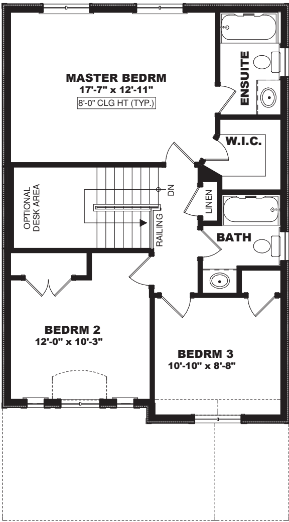
UPPER FLOOR PLAN - 862 SQ. FT
