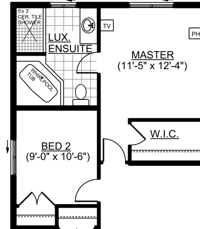
OPTIONAL LUXURY ENSUITE (5015-0095)
