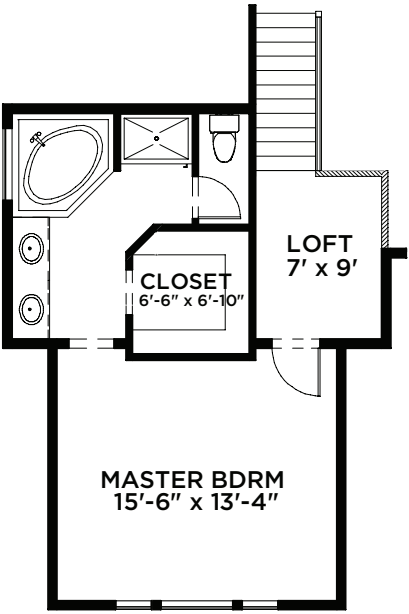
Lofted Master Bedroom & Ensuite
