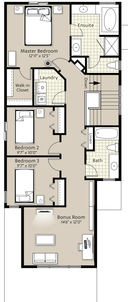
Second Floor | 1140 sq. ft.
