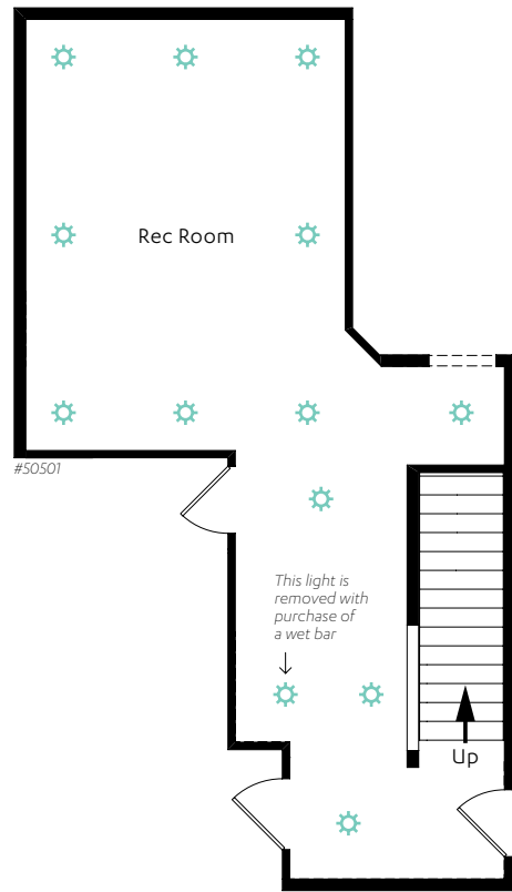
36 Pot Light Basement Development Option Layout*: -6" LED pot lights including dimmer switch
