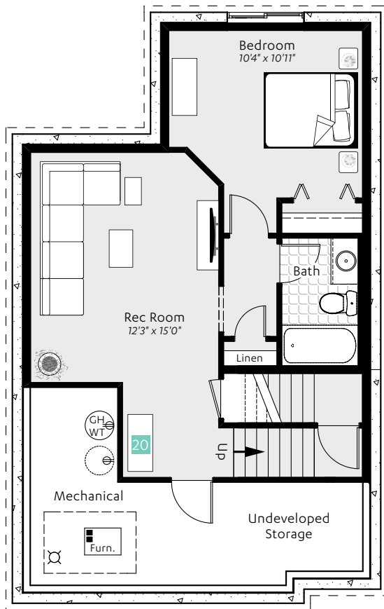
Basement Development Option Level 1 545 sq. ft.
