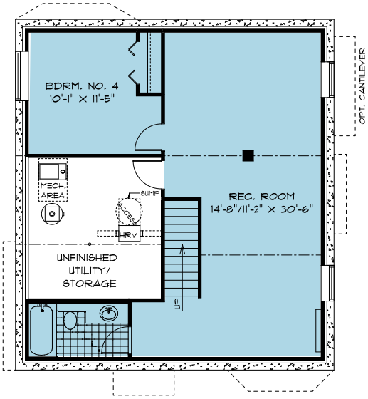
OPTIONAL LOWER LEVEL FLOOR PLAN ( FINISHED AREA 663 SQ. FT. )
