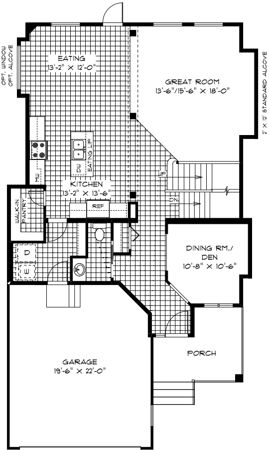
MAIN FLOOR PLAN ( 1152 SQ. FT. ) ADD 9 SQ. FT. FOR OPT. EATING ALCOVE
