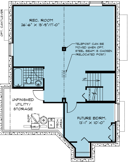
OPTIONAL LOWER LEVEL FLOOR PLAN ( FINISHED AREA 144 SQ. FT. )
