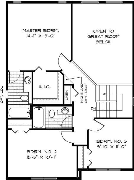
SECOND FLOOR PLAN ( 889 SQ. FT. )
