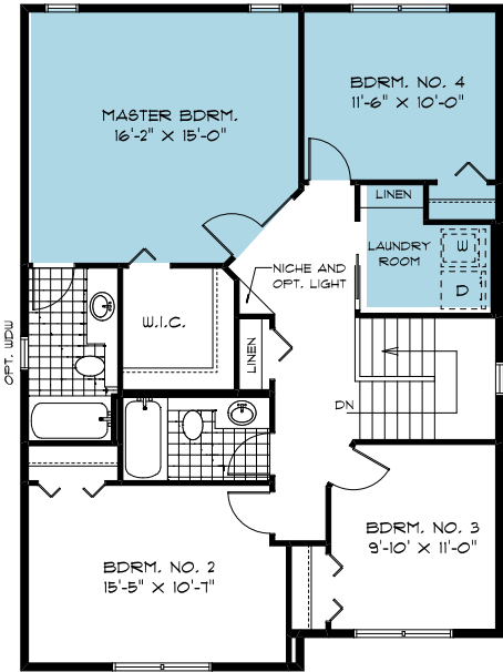
SECOND FLOOR PLAN SHOWN WITH OPT. 4TH BDRM. & LAUNDRY ROOM ( 1136 SQ. FT. )
