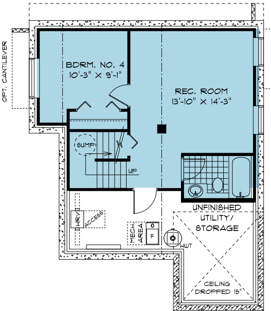
OPTIONAL LOWER LEVEL FLOOR PLAN ( FINISHED AREA 414 SQ. FT. )
