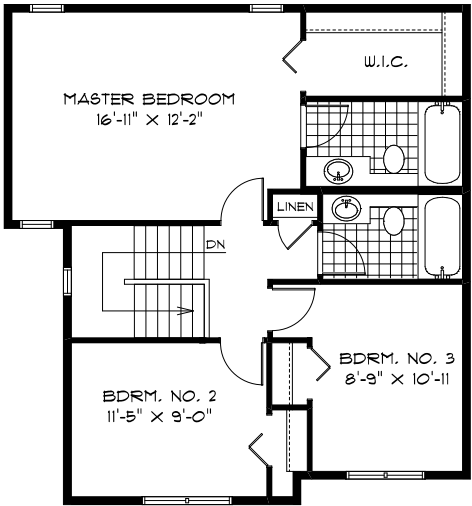
SECOND FLOOR PLAN ( 739 SQ. FT. )
