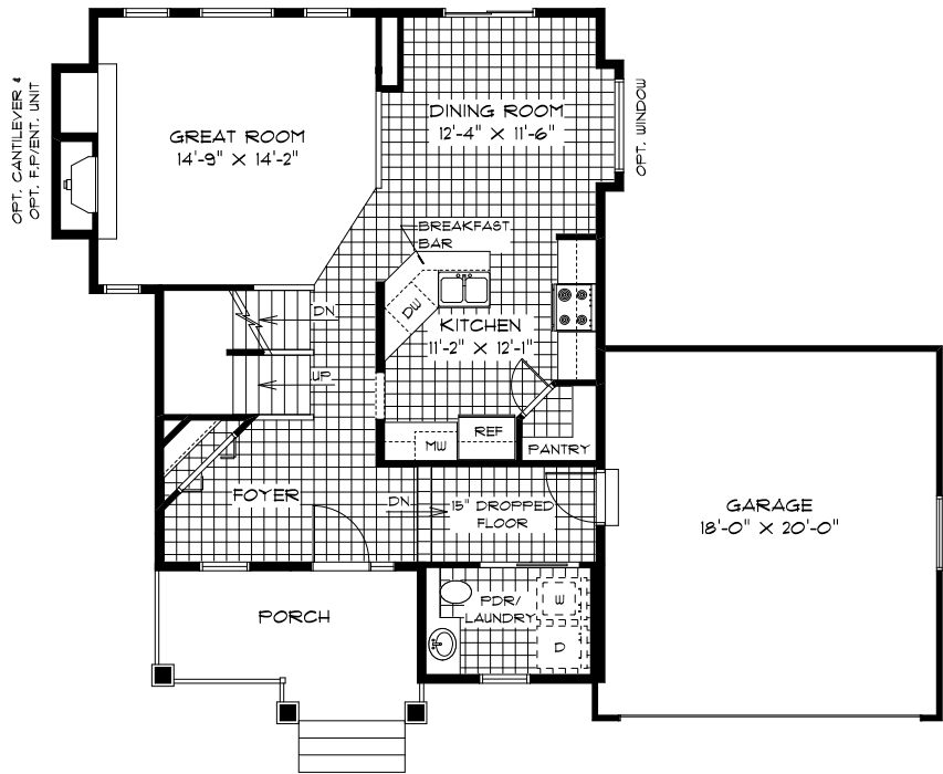
MAIN FLOOR PLAN ( 840 SQ. FT. )
