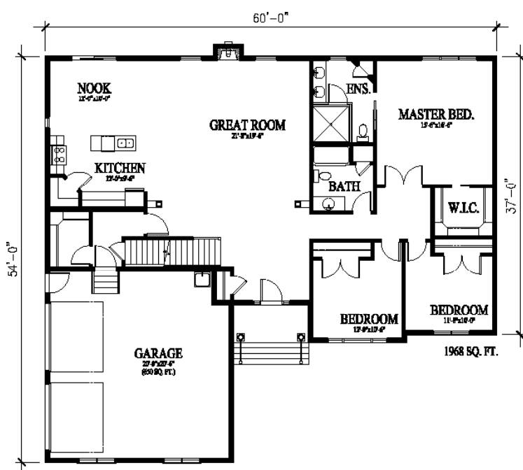
MAIN FLOOR
