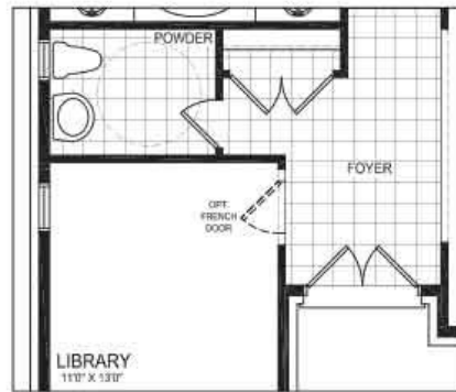
PARTIAL GROUND FLOOR W/ ACCESSIBLE POWDER ROOM STYLE A STYLE B & C SIMILAR
