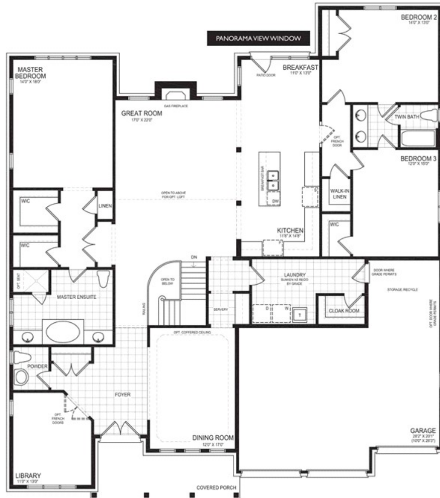
MAIN FLOOR STYLE A
