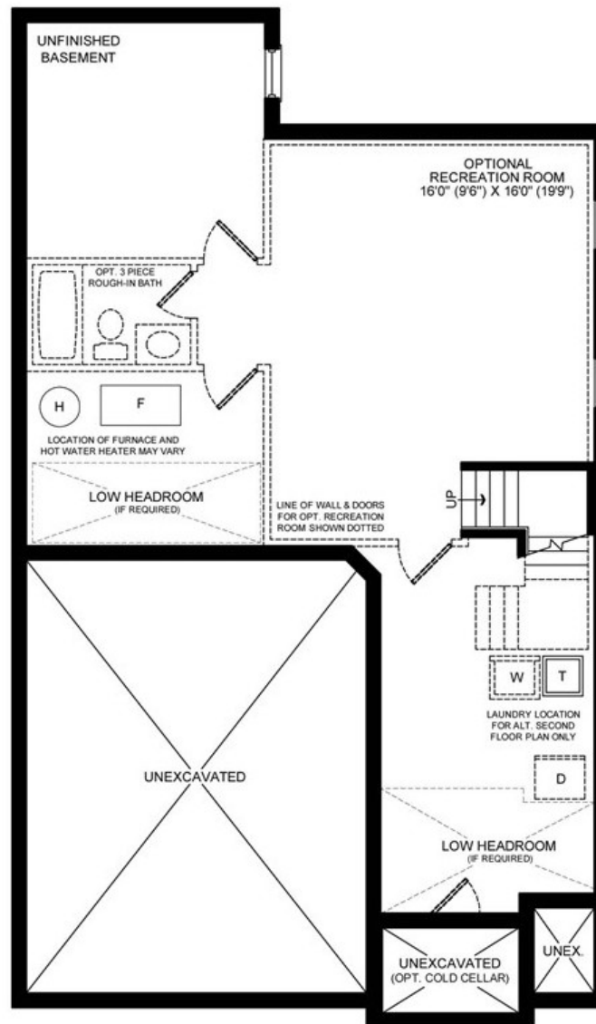
BASEMENT FLOOR STYLE 'A'
