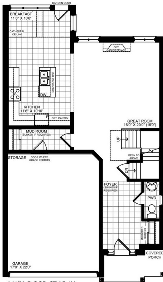
MAIN FLOOR STYLE 'A'
